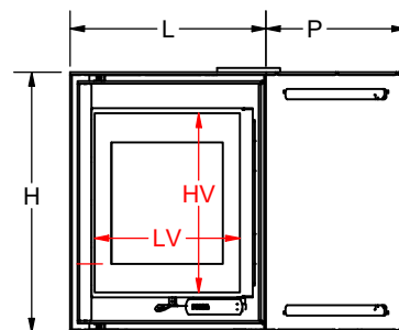
MODBOX50
